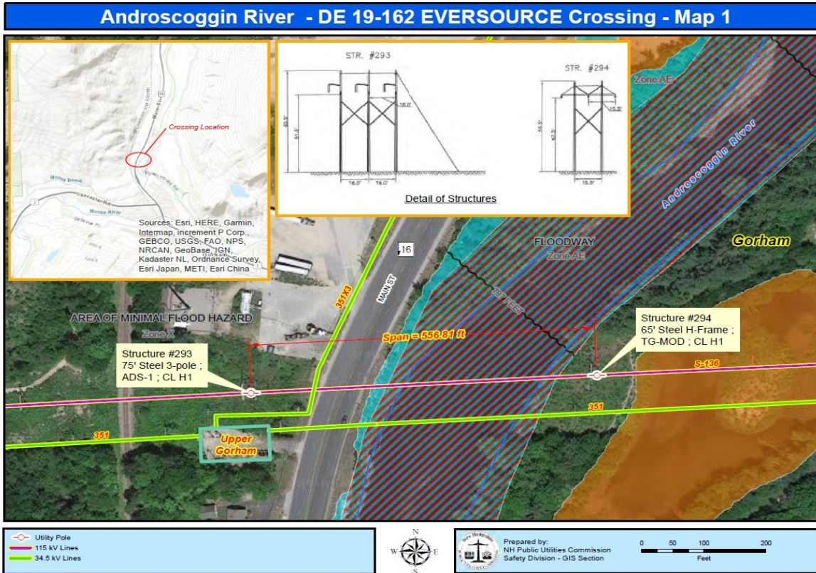
Figure 2: 115kV line, designated as the S 136 Transmission Line, is a span of approximately 557 feet between structures # 293 and # 294, across the Androscoggin River in the Town of Gorham, NH. Of which 243.5 feet crosses the public water way.
