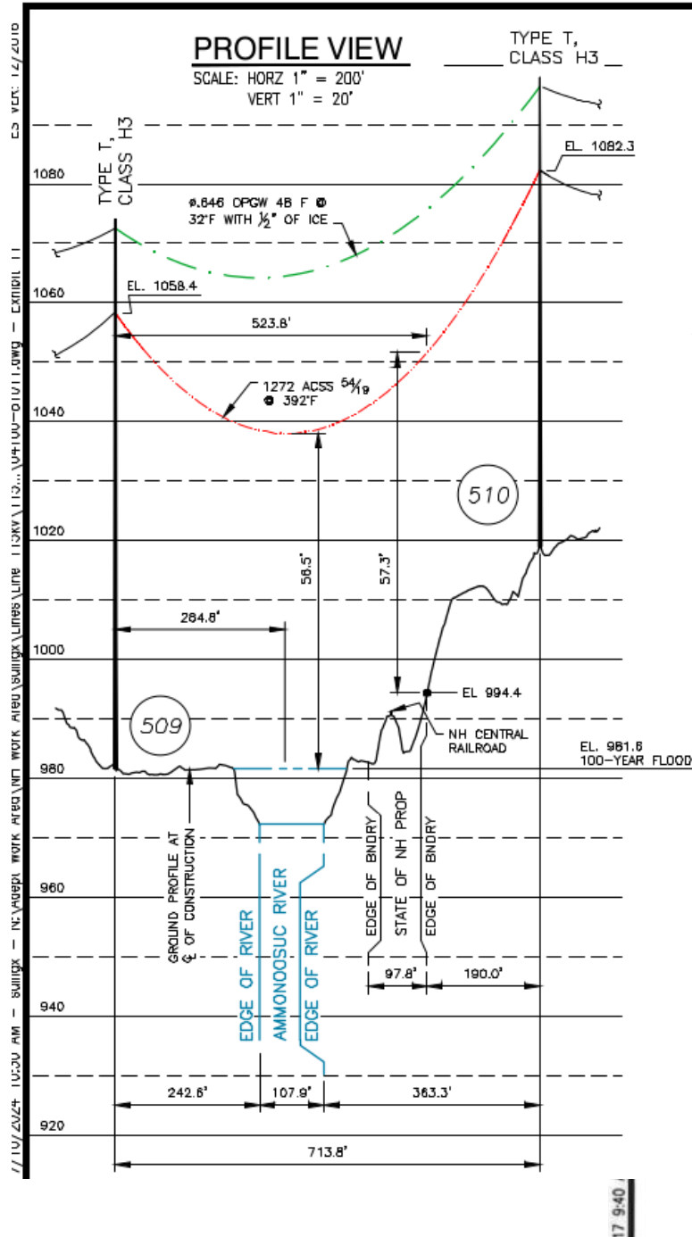
Proposed Ammonoosuc River Crossing
